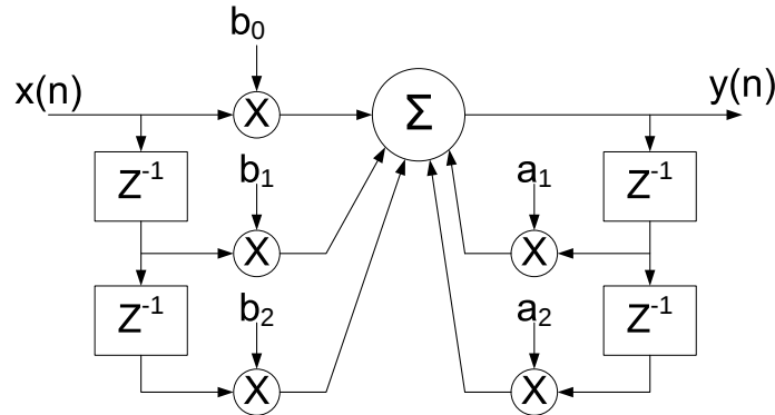
Figure 21. Biquad Filter Configuration
